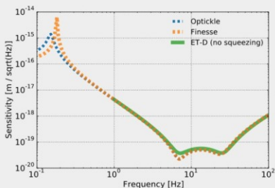
Figure: Almost matching sensitivity curves with different tools, but no squeezing yet
