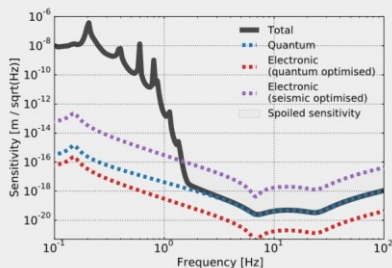
Figure: How do we optimise for both seismic and quantum noise?
